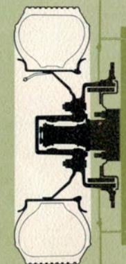
DOUBLE SHIELDED SAFETY BRAKES — Brake drums and linings protected from dirt and water. Extra braking surface for extra safety.
