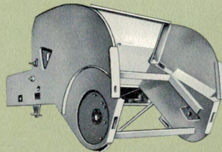
UNITIZED ALL STEEL CHASSIS — Strong . . . "battleship" constructed . . . built-to-last.
